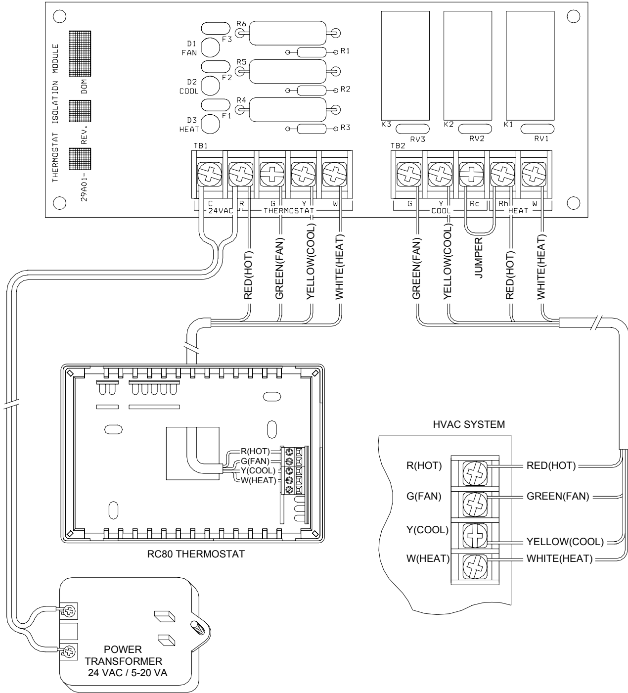
Figure 2 - Connections to Isolate Thermostat from HVAC System
