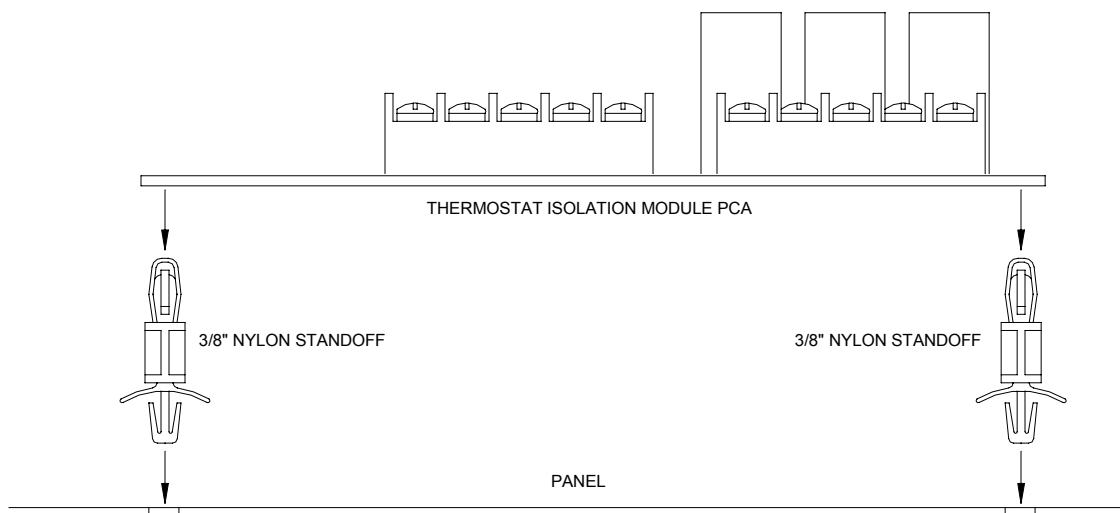
Figure 1 - Mounting the Model 29A00
